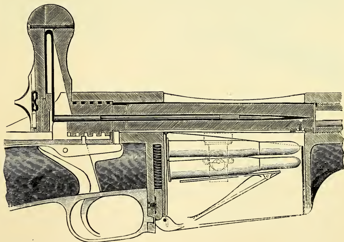
The Marga Repeating Rifle.
